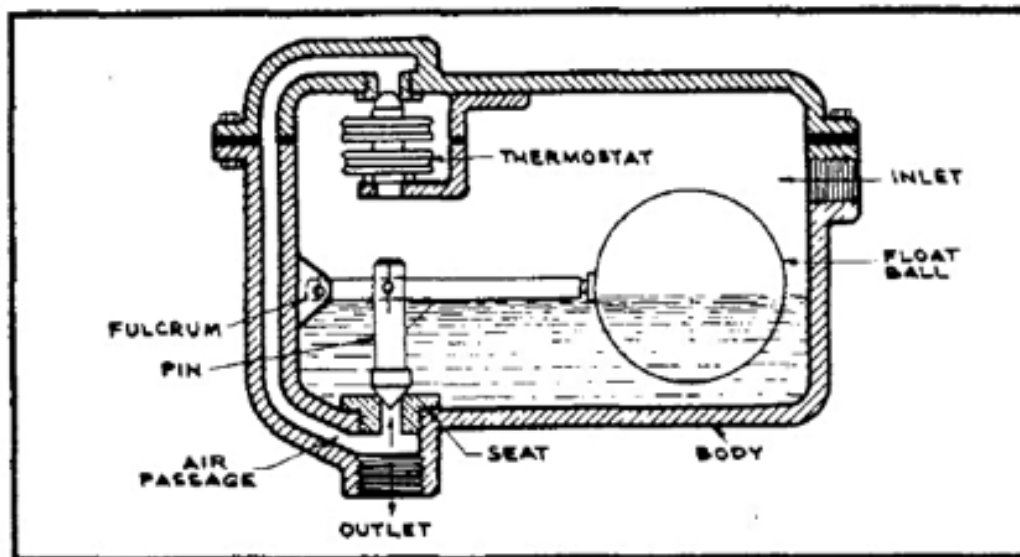
FLOAT AND THERMOSTATIC STEAM TRAP
