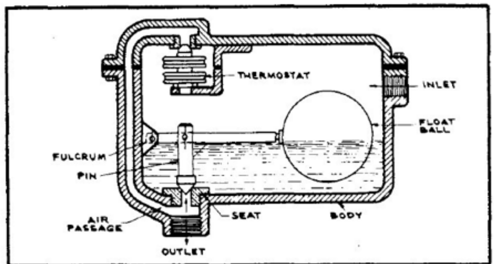
FLOAT AND THERMOSTATIC TRAP
